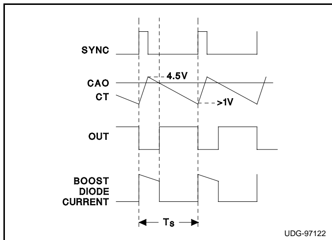
Figure 3a. Oscillator Timing Waveforms Synchronized to Buck (DC/DC) PWM
