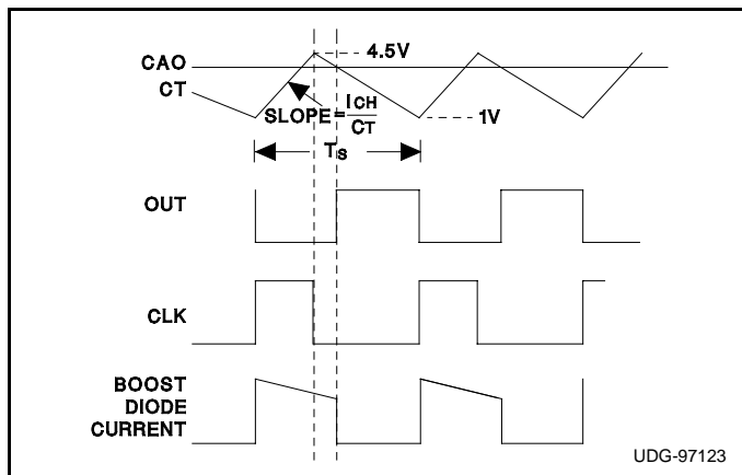
Figure 3c. Frequency Foldback Mode
