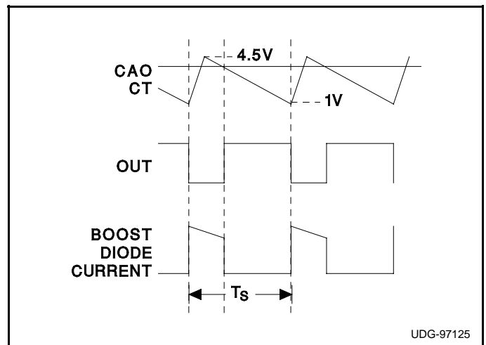
Figure 3b. Oscillator Timing Waveforms Standalone Operation
