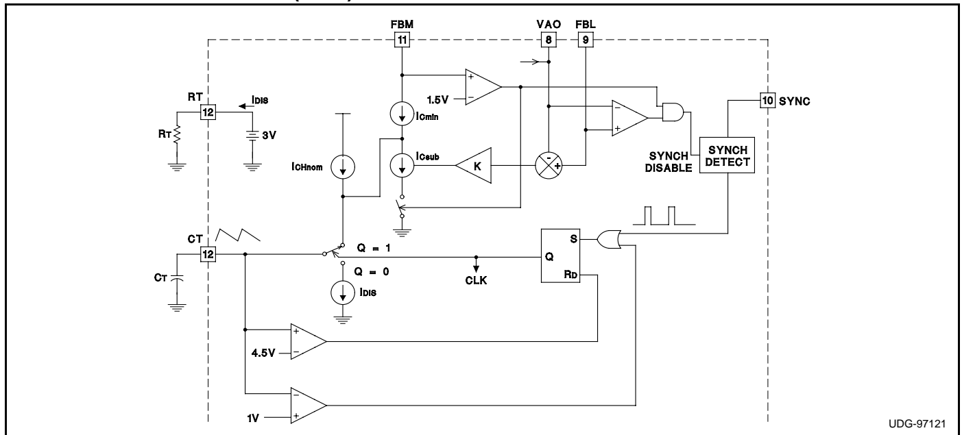
Figure 2. Oscillator Block Diagram
